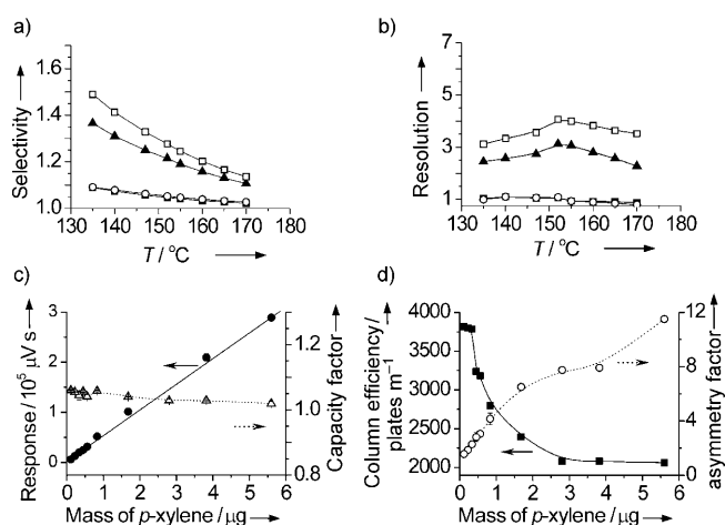
Figure 3. Parameters affecting the separation of xylene isomers and EB: a) effect of temperature on selectivity; \square o -xylene/ m -xylene, \blacktriangle o -xylene/ethylbenzene, \circ ethylbenzene/ m -xylene, \blacksquare m -xylene/ p -xylene; b) effect of temperature on resolution, symbols see panel (a); c) effect of analyte mass on the peak area response ( \bullet ) and capacity factor ( \Delta ); and d) effect of analyte mass on column efficiency ( \blacksquare ) and asymmetry factor ( \circ ). The asymmetry factor is defined as the distance from the center line of the peak to the back slope divided by the distance from the center line of the peak to the front slope, with all measurements made at 10% of the maximum peak height. All experiments were performed at a \text{N}_2 flow rate of 2.3 \text{mL min}^{-1} .
