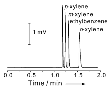
Figure 1. GC separation of xylene isomers and EB on a MIL-101 coated capillary column (15 m long \times 0.53 mm i.d.) at 160°C under a N_2 flow rate of 3 mL min −1 . The mass of each isomer is 350 ng.
