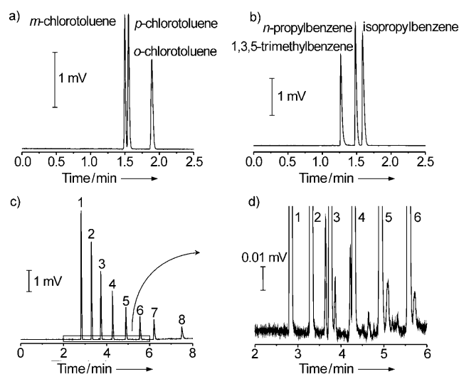
Figure 4. GC chromatograms on the MIL-101 coated capillary column (15 m long \times 0.53 mm i.d.) for the separation of a) m -, p -, and o -chlorotoluene (890 ng each) at a N 2 flow rate of 3 mL min -1 under 160 °C; b) 1,3,5-trimethylbenzene, n -propylbenzene, and isopropylbenzene (1.0 \mu g each) at a N 2 flow rate of 3 mL min -1 under 160 °C; and c) n -alkanes (1: hexane; 2: heptane; 3: octane; 4: nonane; 5: decane; 6: undecane; 7: dodecane; 8: tetradecane) using a three-step temperature program: 60 °C for 0.2 min, then 20 °C min -1 to 200 °C, and finally 200 °C for the remainder of the measurement; d) expanded view of (c) showing the high-resolution separation of the impurities in the n -alkanes mixture.
